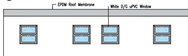
C ELEVATION 1:100@A3
